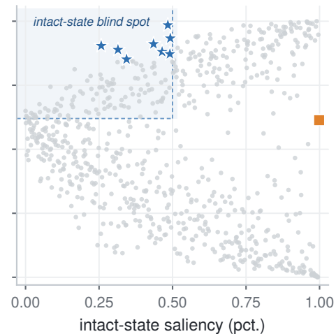
GPT-2-large (774M)
