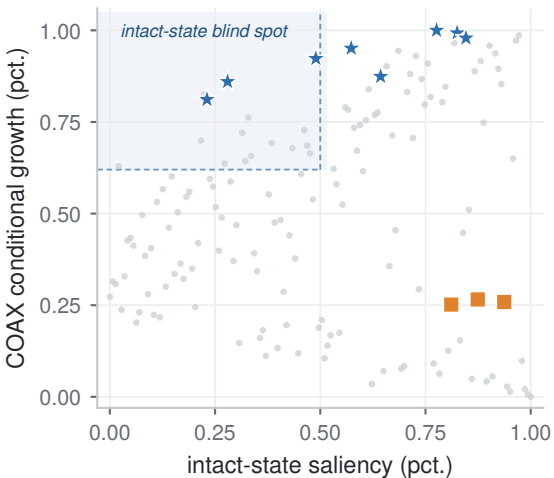
GPT-2-small (124M)
